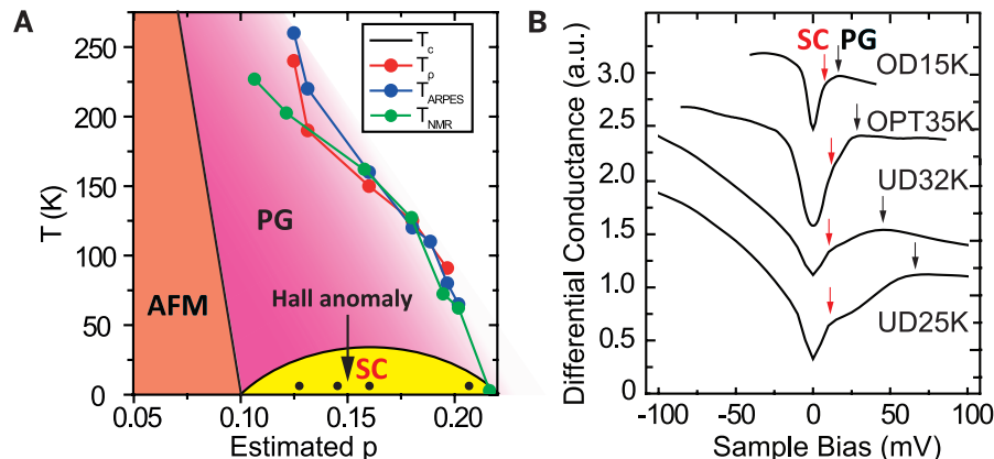
Fig. 1. Phase diagram and spectra. (A) Schematic temperature-doping phase diagram of Bi2201, showing antiferromagnetic insulator (AFM), superconductor (SC), and PG phases. Four black points represent the sample batches of this study, namely underdoped UD25K and UD32K, optimal OPT35K, and overdoped OD15K. The PG transition line T^* is plotted as measured by ARPES (12), resistivity (12) and nuclear magnetic resonance (13). Anomaly in the Hall coefficient (28) is marked by a black arrow. (B) The spatially averaged differential conductance g(E) for each sample. The PG edge is marked with black arrows, whereas the low-energy kink in each spectrum, considered to be related to the superconducting gap (14, 15), is marked with red arrows. a.u., arbitrary units.
