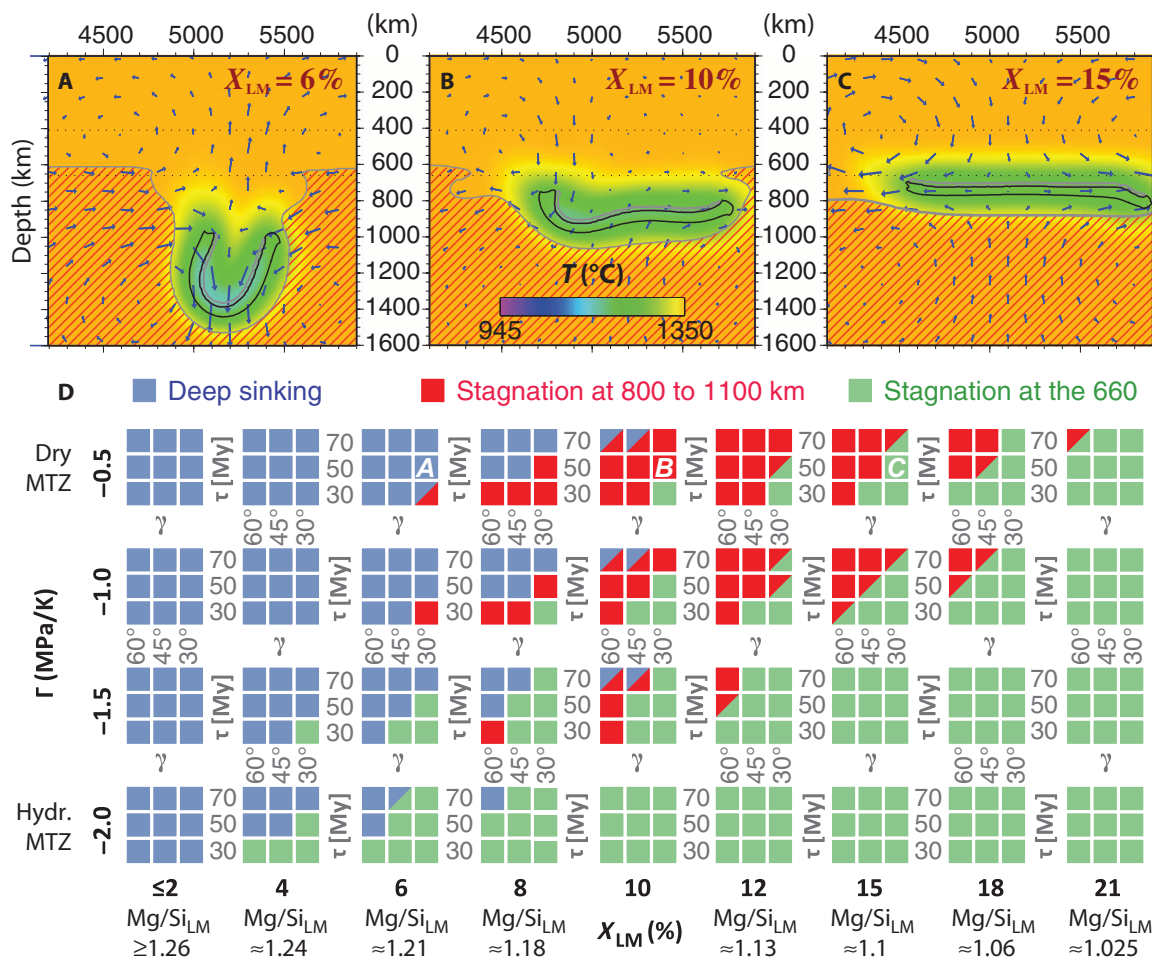
Fig. 3. Numerical-model predictions for three regimes of slab-sinking behavior. (A to C) Arrows denote velocity vectors and colors indicate potential temperature in snapshots at 150 Myr (for time series, see fig. S3). The 5% iso-contours of harzburgite (black) and basalt fraction (gray) are labeled. Domains with X_{LM} > 0 are shown with dark red hatching. Slab-sinking behavior varies as a function of X_{LM} (as annotated) between the cases shown. (D) Map of slab-sinking regimes as a function of all parameters. Mantle parameters \Gamma and X_{LM} are varied between big squares; slab parameters \tau and \beta are varied between small squares (that is, within each big square). Cases (A to C) are labeled. For \Gamma = -3 MPa/K, slabs are always predicted to stagnate at the 660 (not shown). Bottom scale: Mg/Si of the lower mantle, calculated from X_{LM} [according to Workman and Hart (2)].
