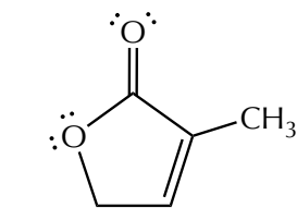
3-methyl-2(5H)-furanone
