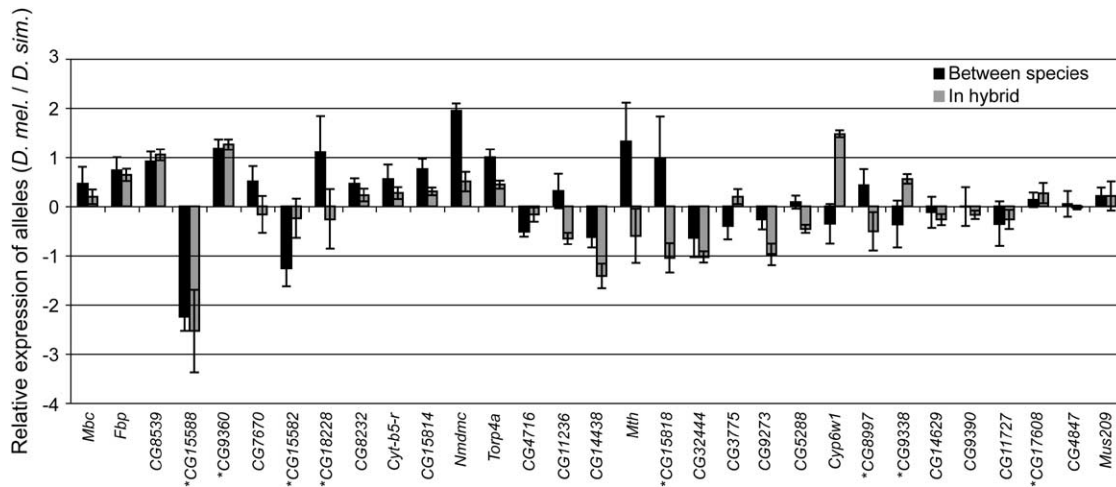
FIGURE 1.—Ratios of allelic expression ( \log_2 ) between species and in the hybrid background for the 31 genes studied. Error bars indicate 95% confidence intervals. Genes are grouped by the inferred patterns of divergence. Mbc , fbp , CG8539 , CG15588 , and CG9360 show divergence in cis . CG7670 , CG15582 , and CG18228 show divergence in trans . CG8232 , Cyt-b5-r , CG15814 , Nmdmc , Torp4a , and CG4716 show divergence in cis and in trans ( cis + trans ). The remainder, except mus209 and CG4847 , show the cis × trans pattern of divergence. In four of these cases ( CG14629 , CG9390 , CG11727 , and CG17608 ) there was significant cis divergence but this divergence was not significantly different from the species divergence, which itself is not different from 0. CG4847 shows neither divergence between species nor cis divergence. Mus209 shows divergence between species but no significant trans effect as detailed in the model. Genes studied previously by WITTKOPP et al. (2004) are indicated with *.
