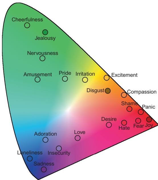
Figure 4. TK's emotion-color associations overlaid on a CIE color-space schematic. [To view this figure in color, please visit the online version of this Journal.]
