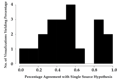
Fig. 2: A histogram showing the number of resample visualizations (out of 20) for different levels of agreement with the single source hypothesis.
