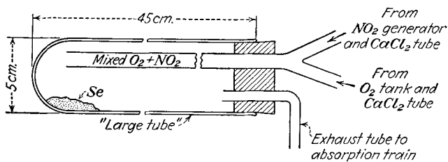
FIG. 22.—Synthesis of selenium dioxide.
