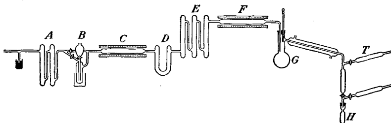
Fig. 6.—Apparatus for synthesis of silicobromoform.
