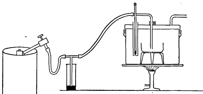
Fig. 14.—Apparatus for preparation of sodium amide.
