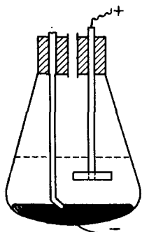
FIG. 1.—Cell for preparation of rare earth amalgams.
