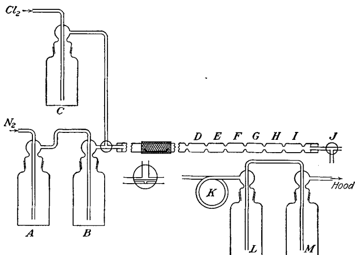
FIG. 31.—Preparation of rhenium pentachloride.
