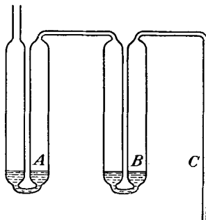
FIG. 13.—U tube for quantitative determination of nitrogen trichloride.
