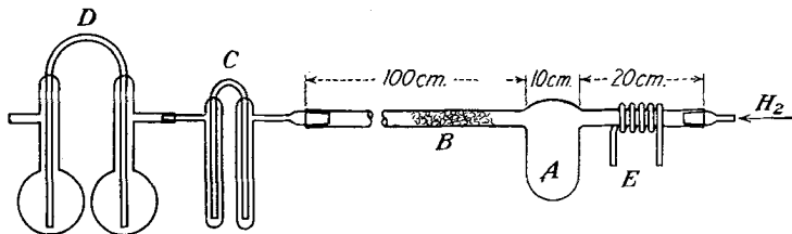
FIG. 30.—Catalytic synthesis of hydrogen iodide.
